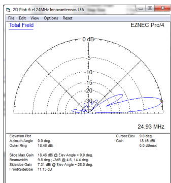
Single 6 element LFA up 12m above ground
