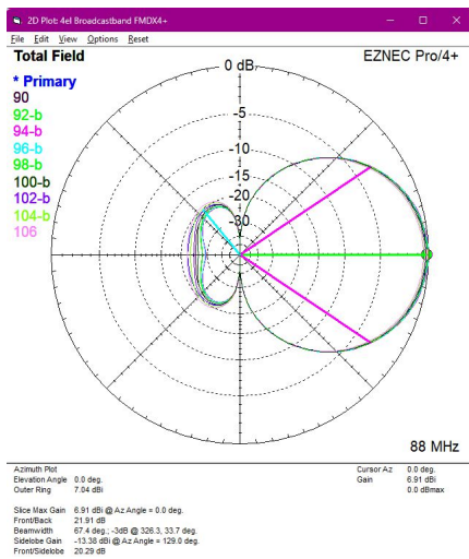
88-108MHz performance plot over-lays showing the impressively consistant performance of the FMDX4+
