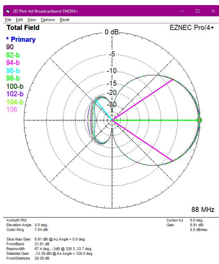
88-108MHz performance plot over-lays showing the impressively consistant performance of the FMDX4+
