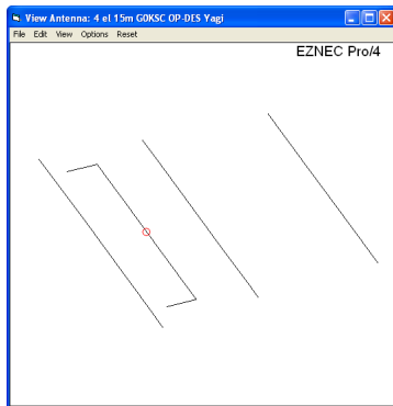
The 4el 21MHz OP-DES Element Layout - how the OP-DES Yagi looks
