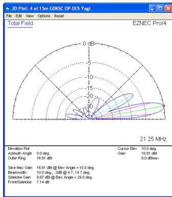
2 x 4el OP-DES Yagi 9m apart with the bottom antenna 15m above ground
