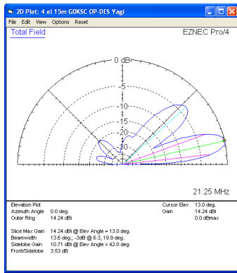
Single 4 element OP-DES up 15m above ground
