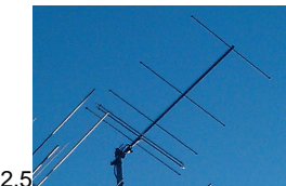
A 5 element OWL (Optimised Wideband Low Impedance) Super-Light Yagi for 69.9-70.5MHz
