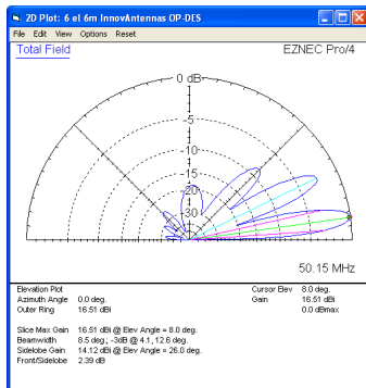
Single 6 element OP-DES up 10m above ground
