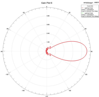
The exceptional elevation plot of the super clean LFA Ultra X-pol Yagi
