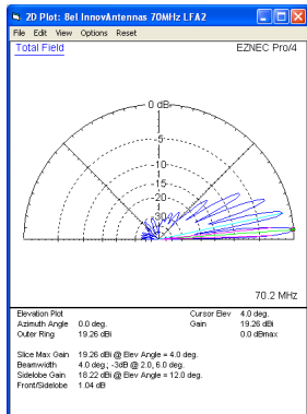
Single 8el 15m above ground
