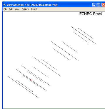
The 28-50-15 Antenna Layout
