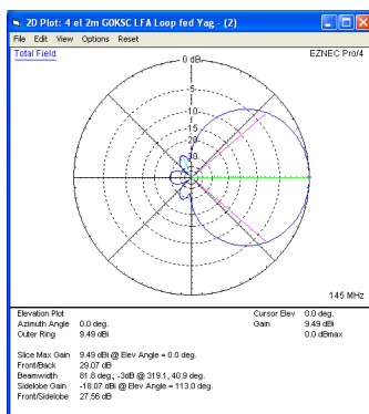
Elevation Plot
