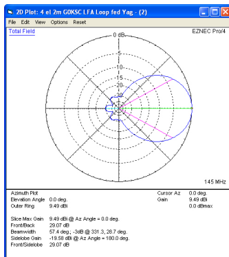
Azimuth Plot
