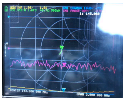
Analyser plot of the 3el Graves LFA at installation - 1.01:1 @ 143.060MHz. The plot also shows a sweep 1MHz either side of this frequency
