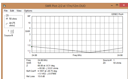
SWR 24MHz
