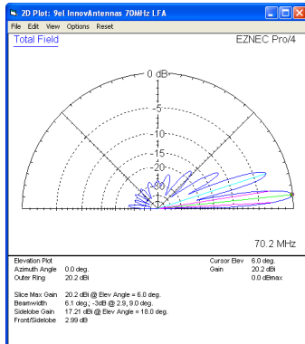
1 x 9el LFA at 10m above ground
