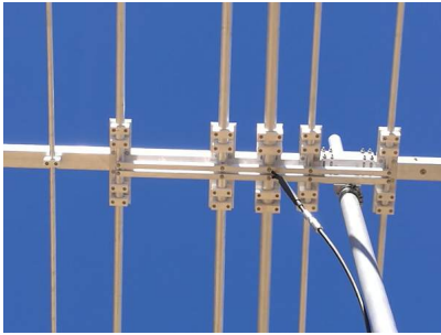
Close-up of the feed arrangement on the XR6 MkII with straight, parrallel lines
