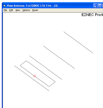
The 4el 28MHz LFA Element Layout
