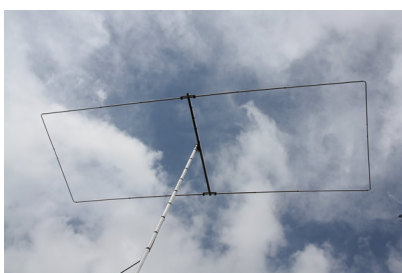
WA2TDE's comments about his 20m Moxon:
