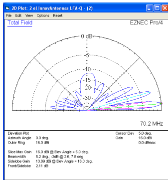
2 x 2 el LFA Yagi 3m apart with the bottom antenna 10m above ground
