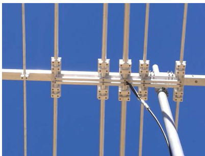
Close-up of the feed arrangement on the XR7 with straight, parrallel lines
